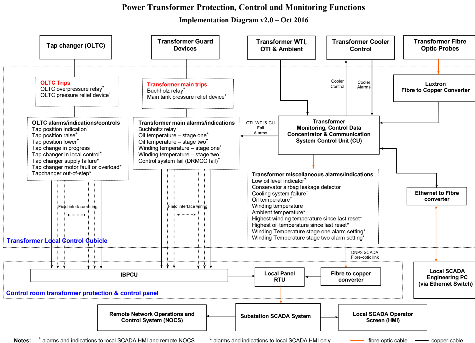
Figure 1 Network Transformer Protection, Control and Monitoring Functions – Implementation diagram v2.0
